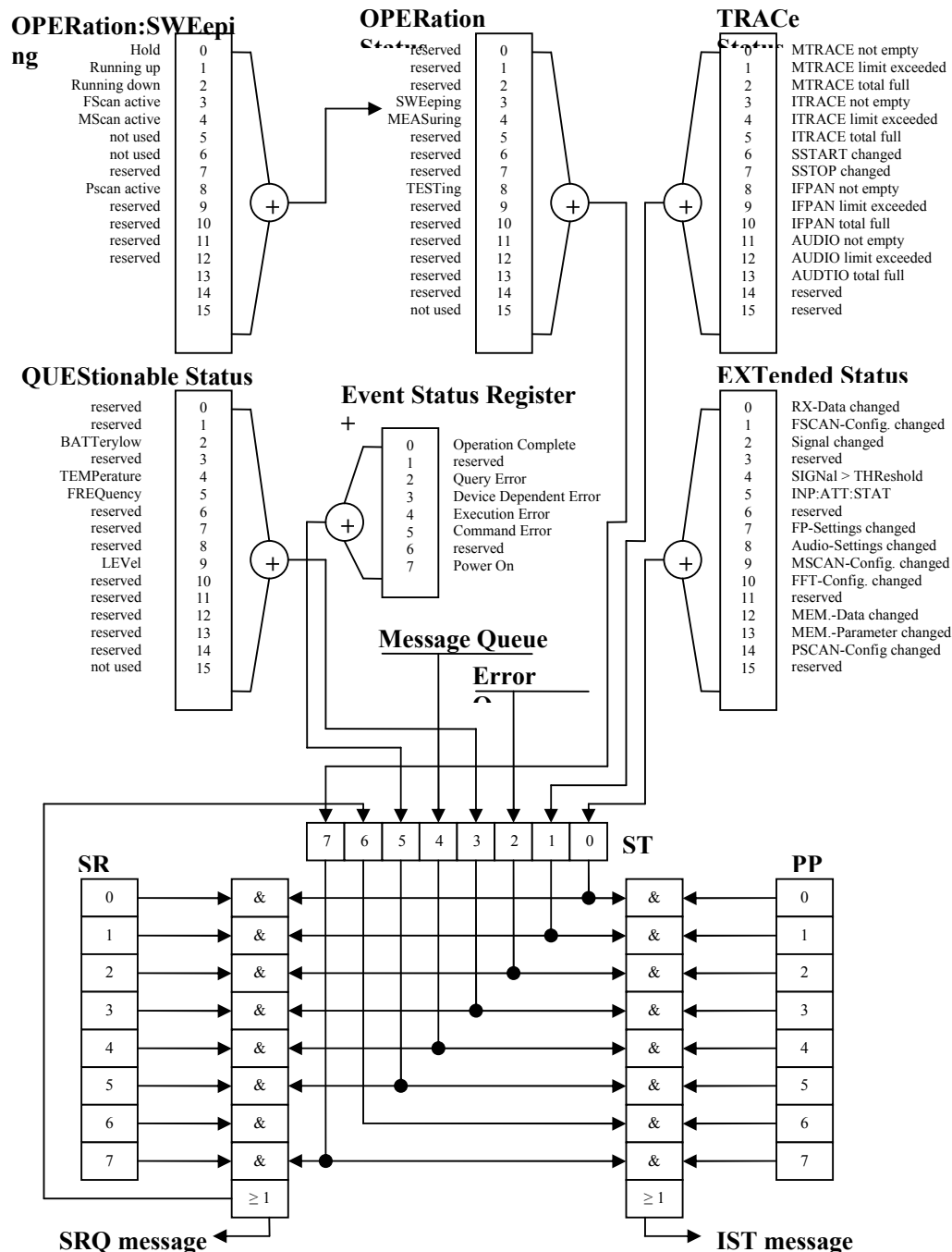
Figure 3: Status Registers
