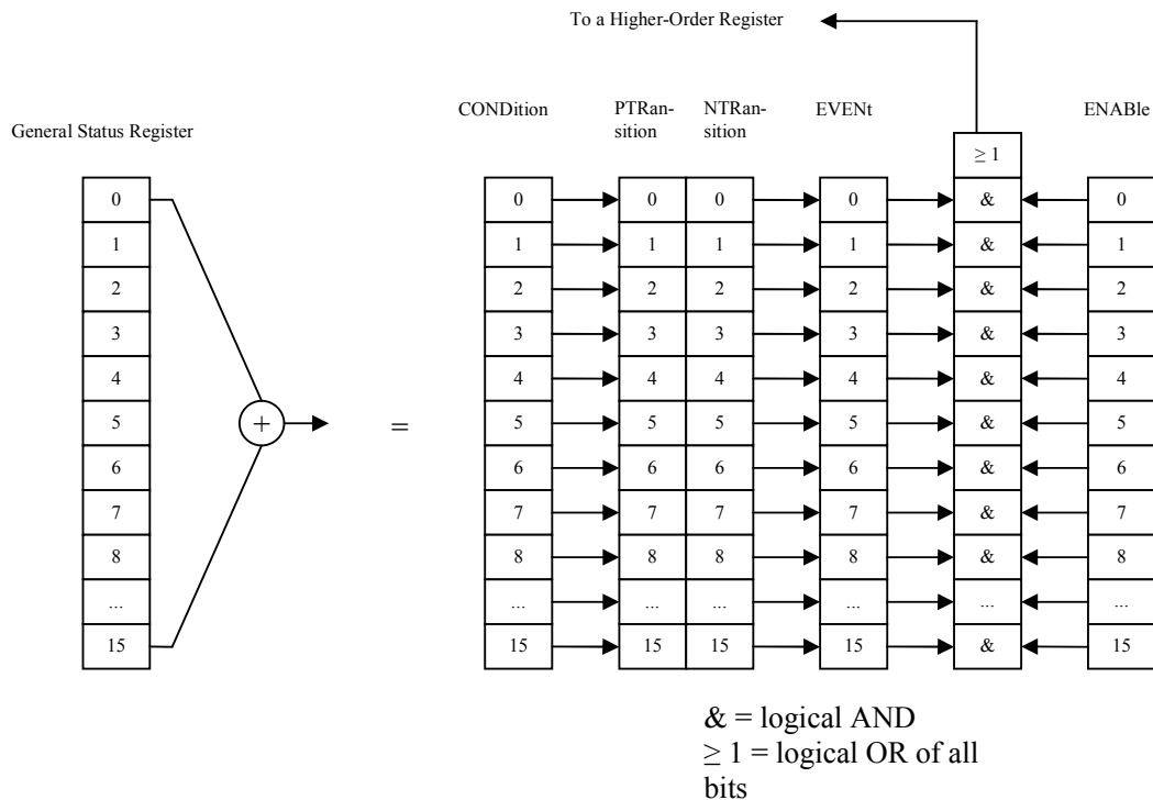
Figure 2: Status Register Model
