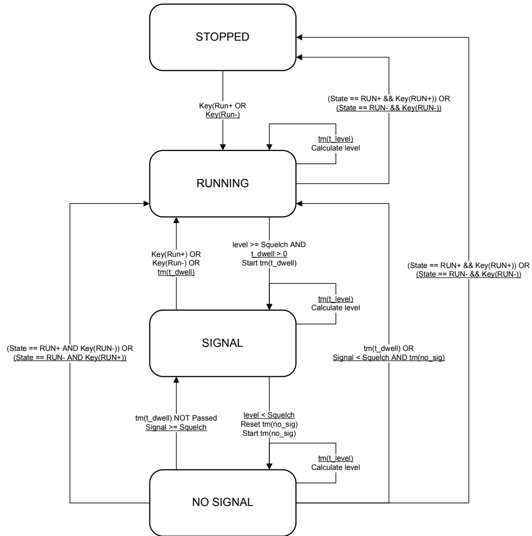
Figure 4 Frequency Scan Mode States
